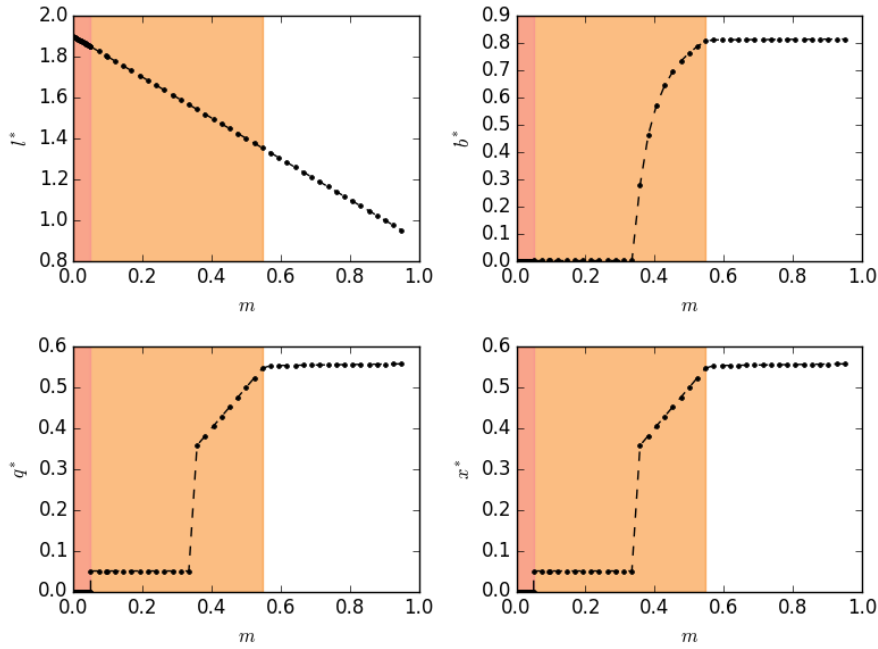
Figure 2: Markov policy functions with \tau = 0.1
