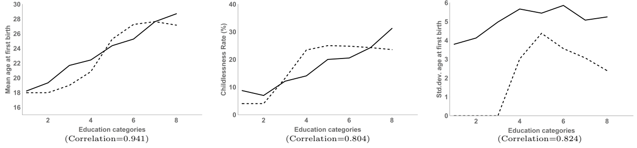
Figure 2: Overidentifying Restrictions: Education Gradient - data:solid, simulated: dashed
