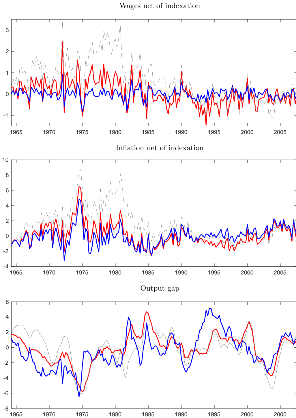
Figure 7: Optimal Policy.
