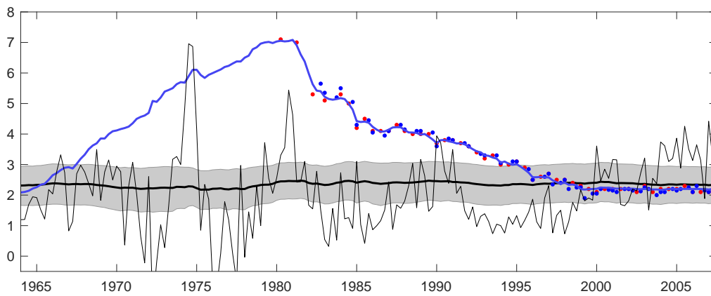
Figure 6: Long-run Inflation expectations.
