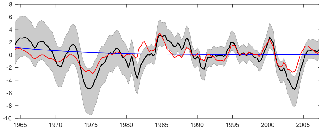
Figure 8: Optimal Policy: output gap without markup shocks
