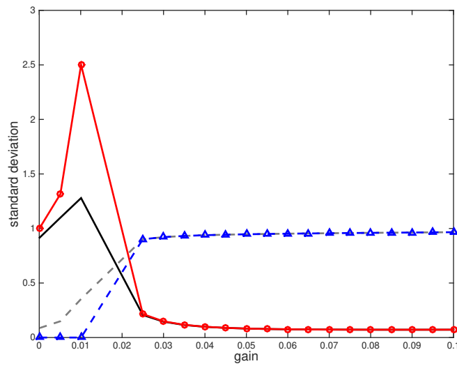
Figure 10: Volatility as a function of the constant gain.
