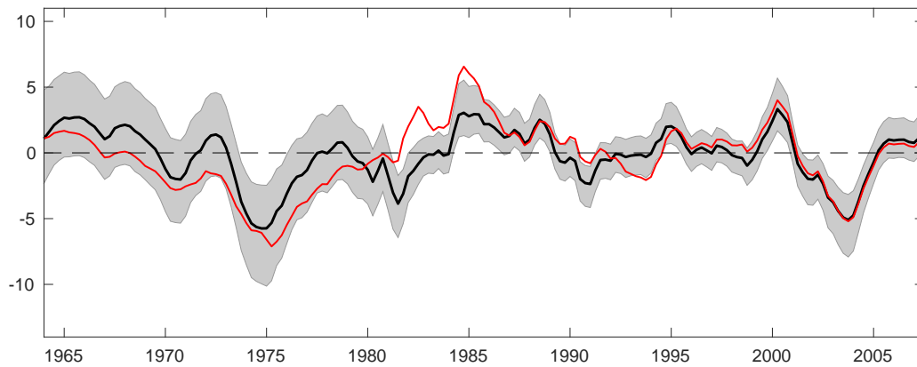
Figure 3: Over-extrapolation and monetary policy.
