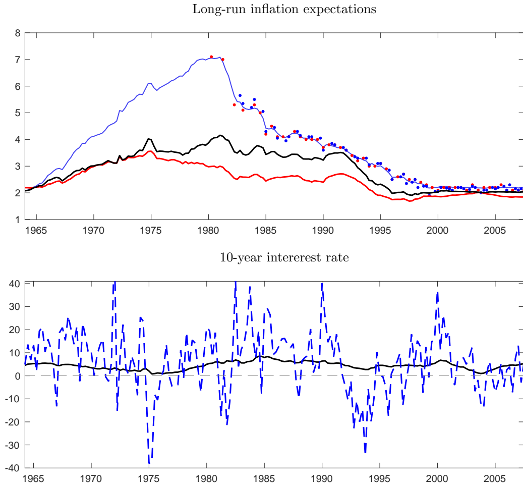
Figure 9: Long-run trends under optimal policy.
