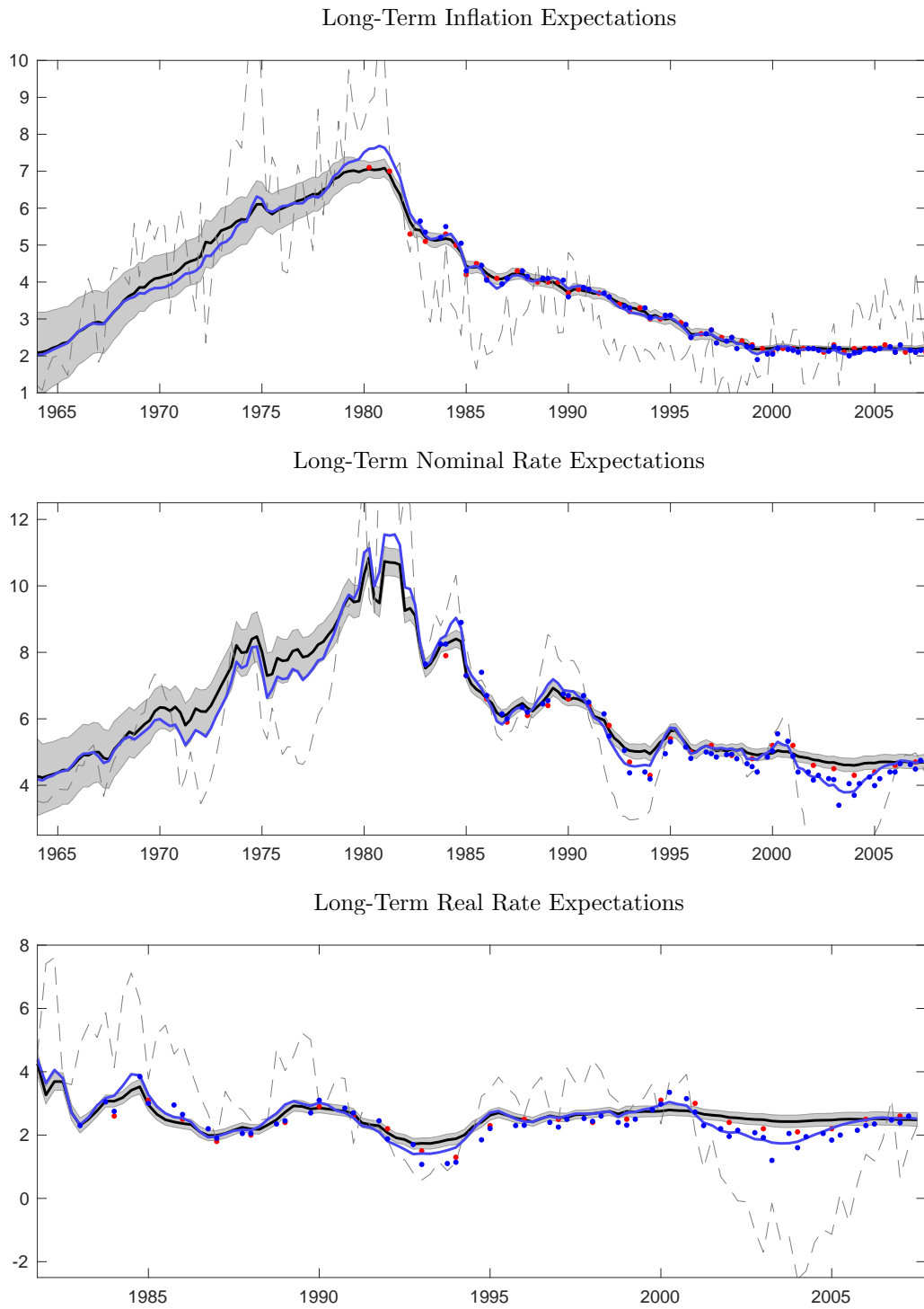
Figure 2: Baseline Predictions.
