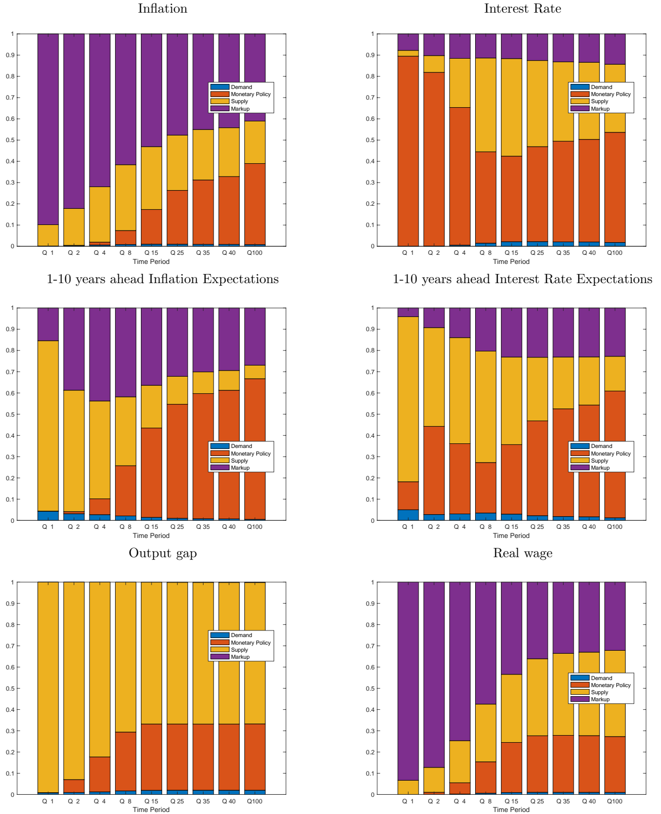
Figure 5: Variance Decomposition
