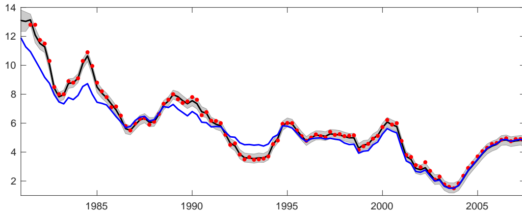
Figure 4: Short-Term interest rate expectations
