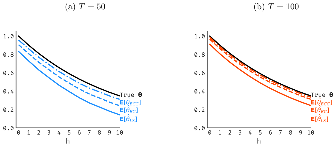
Figure C.3: \hat{\theta}_{BC} and \hat{\theta}_{BCC} are closer than \hat{\theta}_{LS} to \theta , on average, in our LPs without controls when y_t is an AR(1) with \rho = 0.90 .
