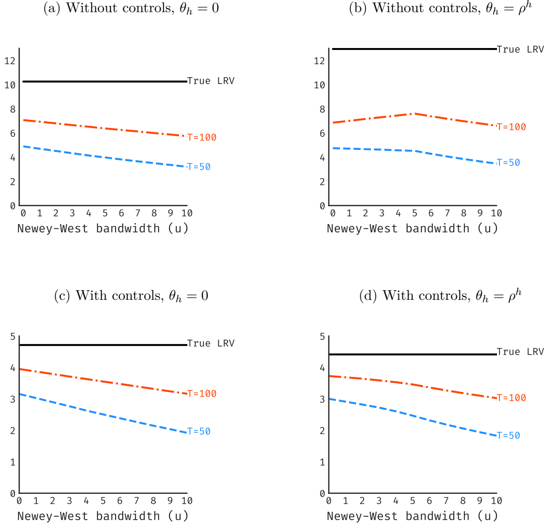
Figure 7: Estimators of standard errors in an LP with h = 5 are biased in empirically-relevant samples when y_t is an AR(1) with \rho = 0.95 .
