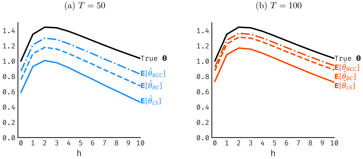
Figure D.3: \hat{\theta}_{BC} and \hat{\theta}_{BCC} are closer than \hat{\theta}_{LS} to \theta , on average, in our LPs without controls when y_t is an AR(1) with \rho = 0.95 and \psi = 0.4 .
