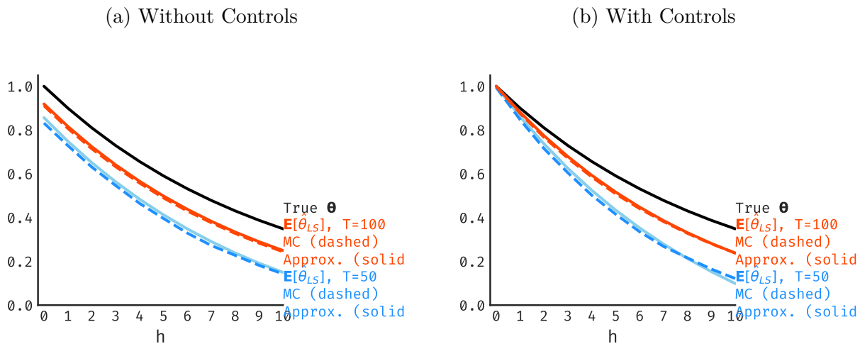
Figure C.2: The bias approximation is accurate in our LPs.
