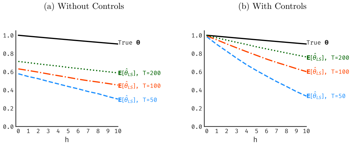
Figure C.5: LP estimators are biased in empirically-relevant samples when y_t is an AR(1) with \rho = 0.99 .
