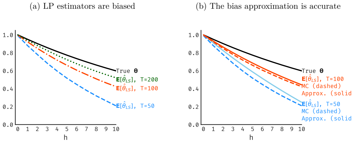
Figure G.1: LP with lag augmentation when y_t is an AR(1) with \rho = 0.95 .
