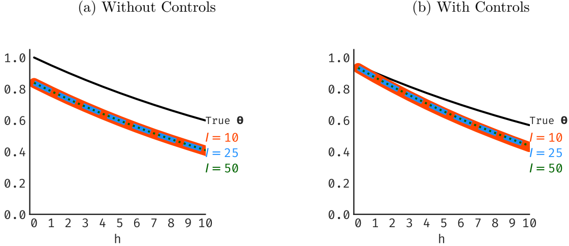
Figure 6: LP estimators without controls are biased in empirically-relevant samples when y_{i,t} is an AR(1) with \rho = 0.95 .
