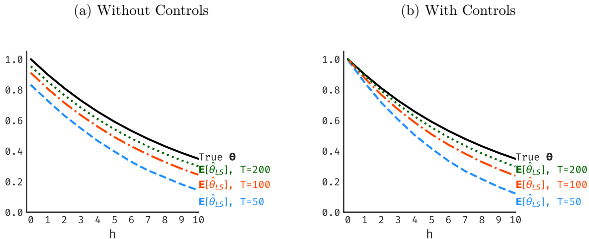
Figure C.1: LP estimators are biased in empirically-relevant samples when y_t is an AR(1) with \rho = 0.90 .
