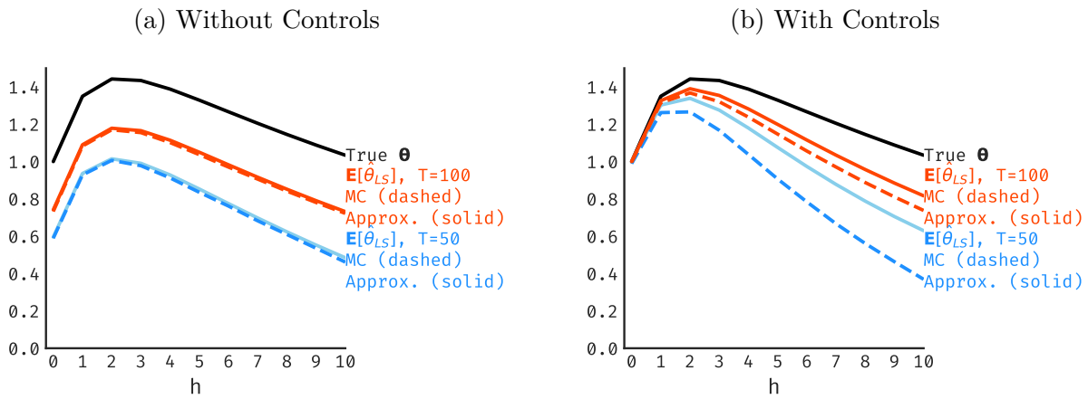
Figure D.2: The bias approximation is accurate in our LPs.
