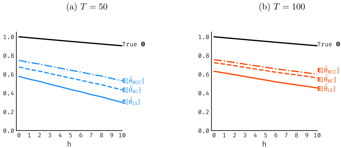
Figure C.7: \hat{\theta}_{BC} and \hat{\theta}_{BCC} are closer than \hat{\theta}_{LS} to \theta , on average, in our LPs without controls when y_t is an AR(1) with \rho = 0.99 .
