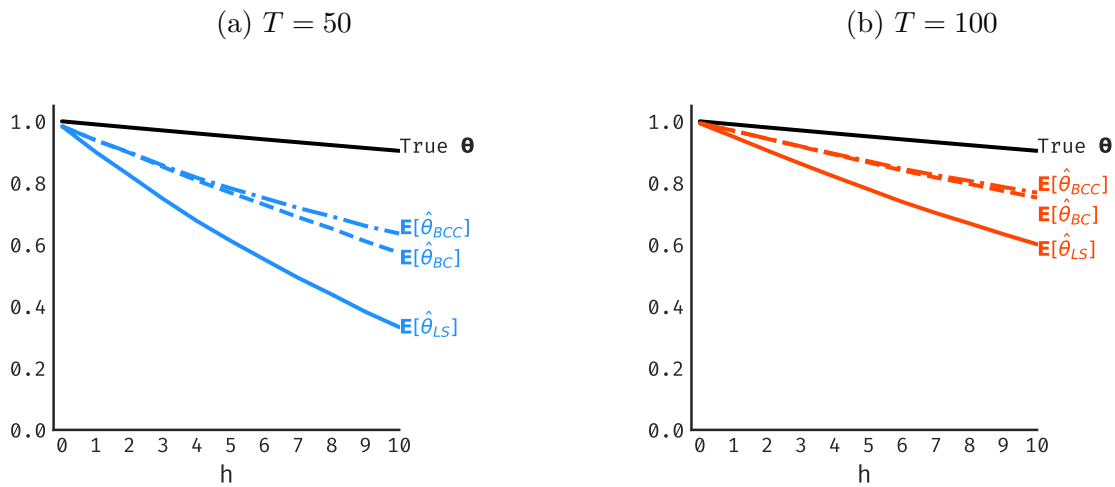
Figure C.8: \hat{\theta}_{BC} and \hat{\theta}_{BCC} are closer than \hat{\theta}_{LS} to \theta , on average, in our LPs with controls when y_t is an AR(1) with \rho = 0.99 .
