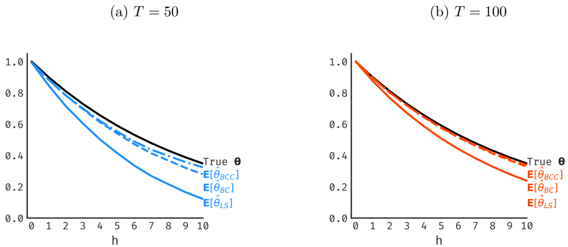
Figure C.4: \hat{\theta}_{BC} and \hat{\theta}_{BCC} are closer than \hat{\theta}_{LS} to \theta , on average, in our LPs with controls when y_t is an AR(1) with \rho = 0.90 .
