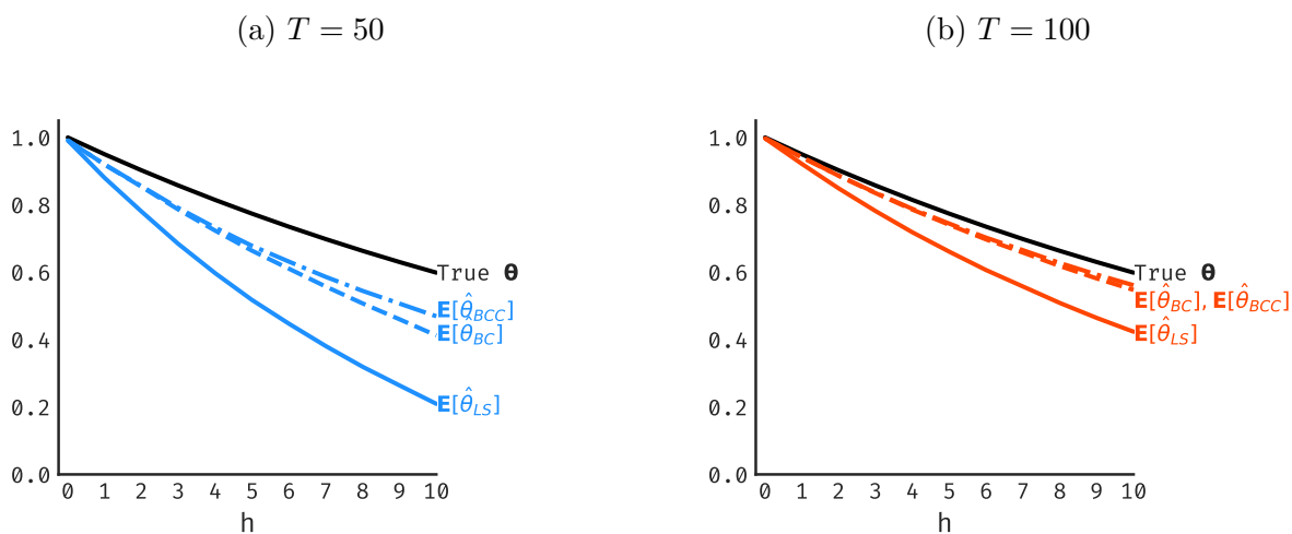
Figure G.2: Bias correction in an LP with lag augmentation when y_t is an AR(1) with \rho = 0.95 .
