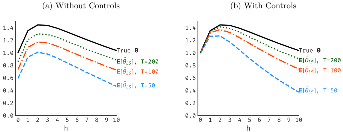
Figure D.1: LP estimators are biased in empirically-relevant samples when y_t is an AR(2) with \rho = 0.95 and \psi = 0.4 .
