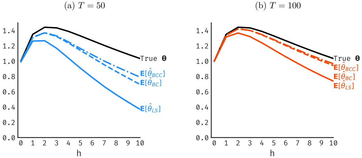
Figure D.4: \hat{\theta}_{BC} and \hat{\theta}_{BCC} are closer than \hat{\theta}_{LS} to \theta , on average, in our LPs with controls when y_t is an AR(2) with \rho = 0.90 and \psi = 0.4 .
