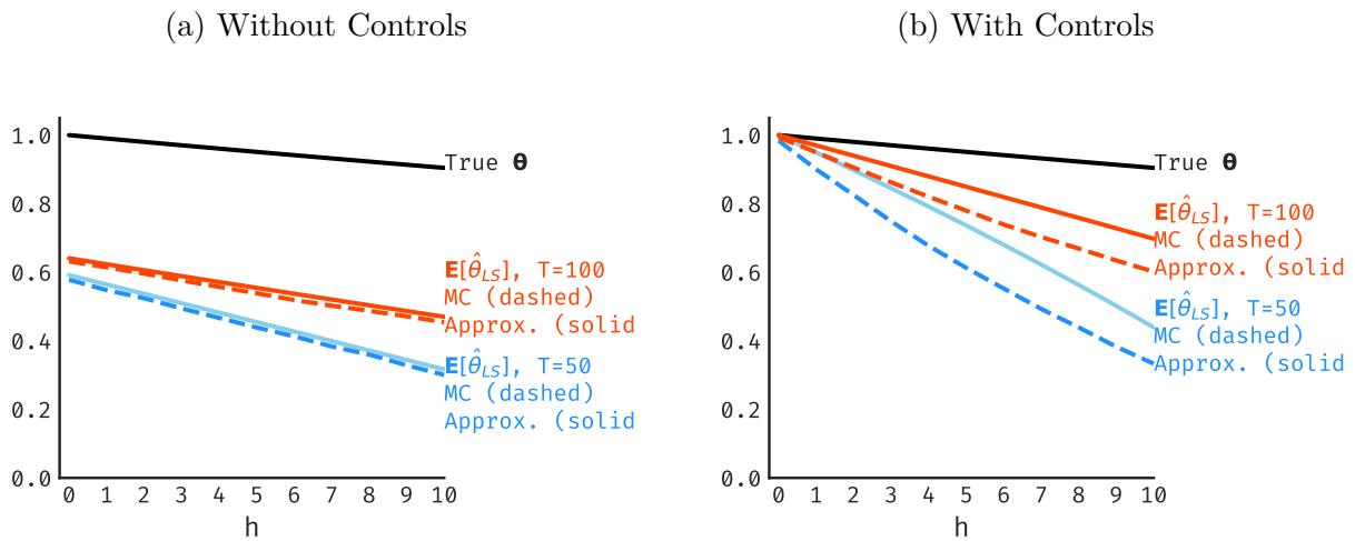
Figure C.6: The bias approximation is accurate in our LPs.
